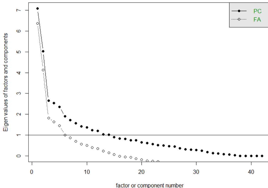
Scree plot
